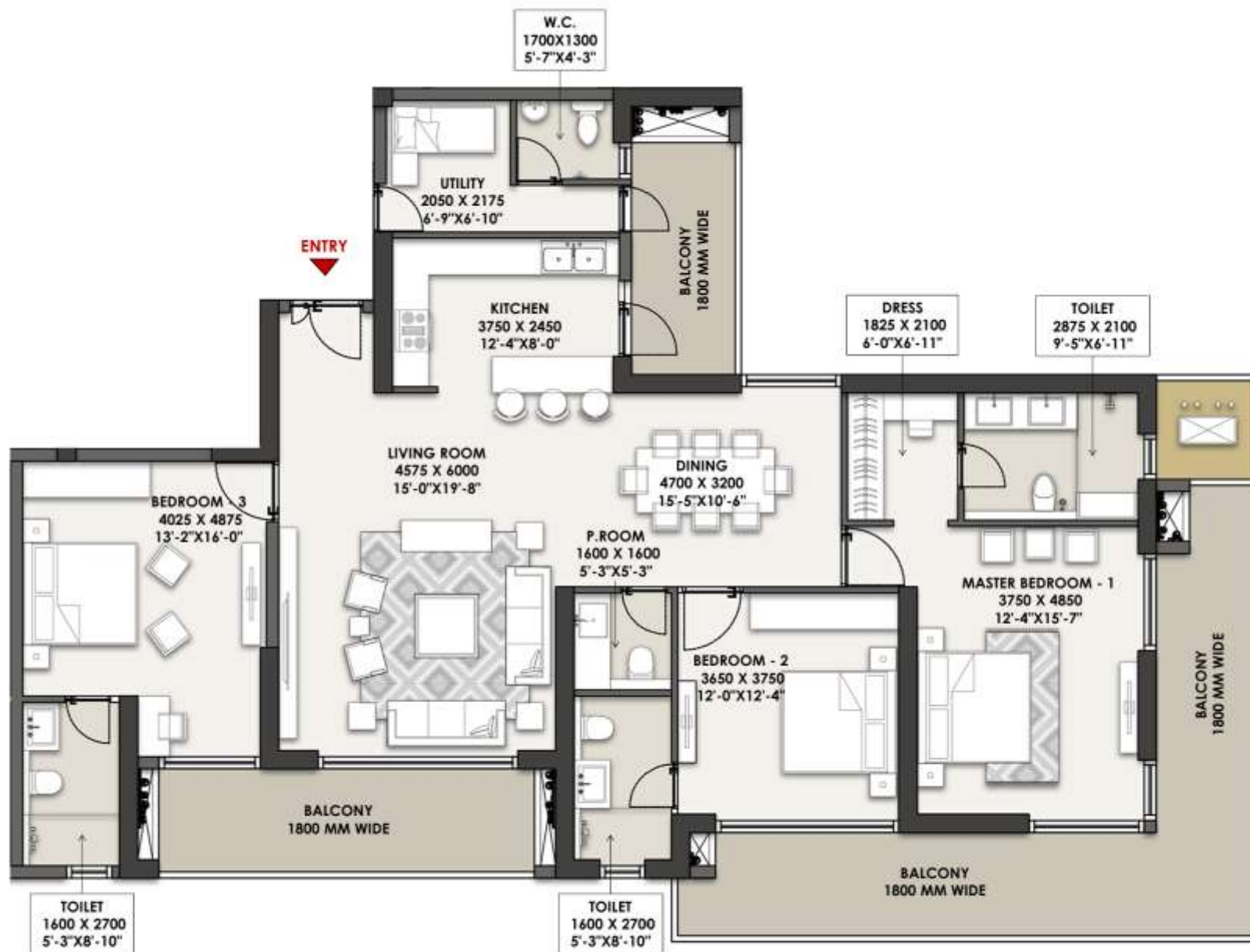
LANDMARK 3 BHK - UNIT PLAN
